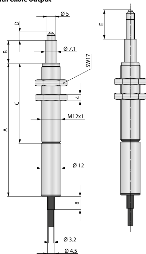
Version with cable output
