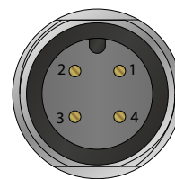
connector M12, male
