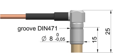
T2-G-KR-VK7 (SHORT VERSION)
