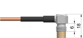
T2-G-KR-VK7 (SHORT VERSION)
