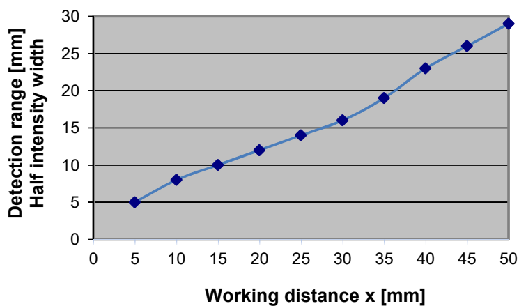
SPECTRO-3-DIL-SL Detection range [mm]
