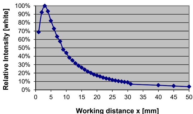
SPECTRO-3-DIL-SL INT [relative]
