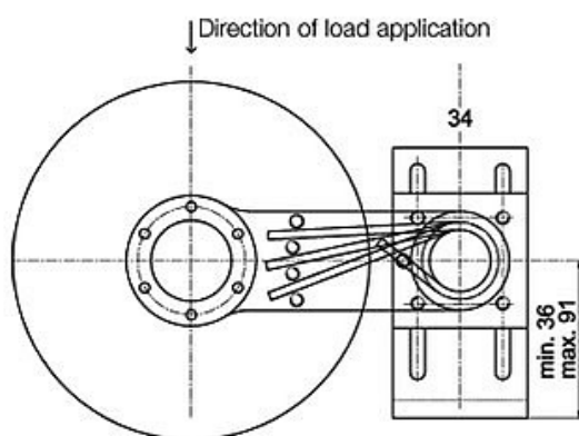
Spring lever, cross section
