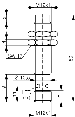
DW-LS-71x-M12
