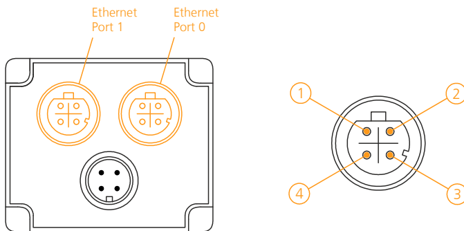
Figure 4: Connection diagram of the Ethernet port 0 & 1
