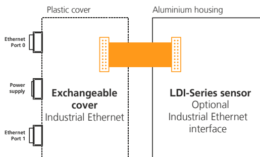
Figure 5: Connection diagram of exchangeable cover with Industrial Ethernet and LDI-Series sensor
