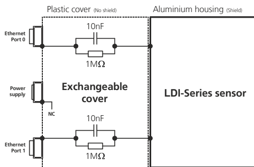
Figure 6: Shielding concept of the LDI-Series sensor and the exchangeable cover with Industrial Ethernet
