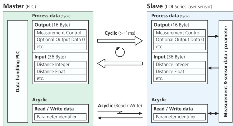
Figure 8: Cyclic (Process data) and acyclic communication between Industrial Ethernet Master (PLC) and the LDI-Series device with Industrial Ethernet interface.
