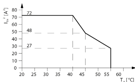
Figure 1 Derating curve
