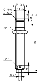
DW-AD-50x-P12-627
