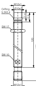
DW-AS-50x-P12-622
