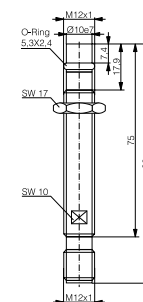
DW-AS-50x-P12-635
