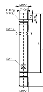
DW-AS-50x-P12-621
