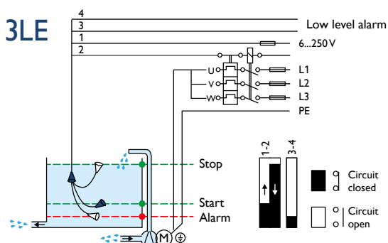
CHARGING-PUMP CONTROL + ISOLATED LOW LEVEL ALARM
