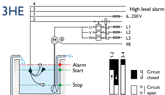
DISCHARGING-PUMP CONTROL + ISOLATED LOW LEVEL ALARM
