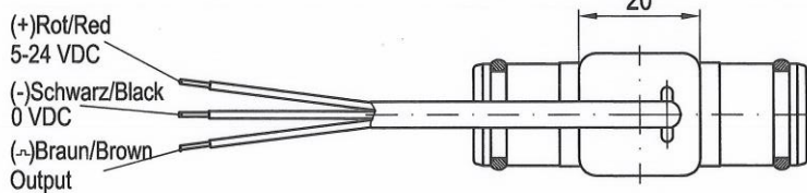
O-Ring, with round cable 3 x AWG 24 and free cable ends
