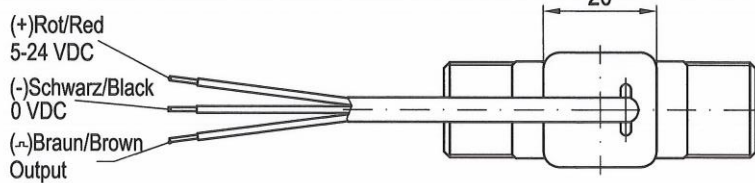
G 3/8" or 3/8" NPT with round cable 3 x AWG 24 and free cable ends
