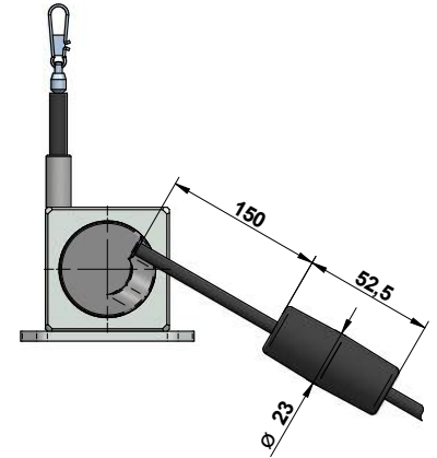
Detailed view: battery integrated in the cable
